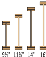
PWI 47 3/8" OSB Web 2 5/16" x 1 1/8" Flange
